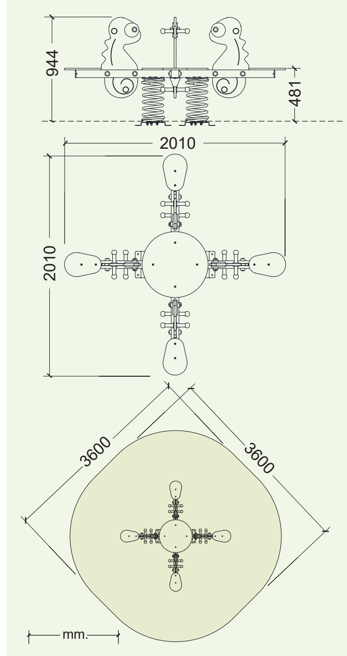
BALANCÍN DE MUELLES "CUARTETO CAMALEONES" (4 PLAZAS) SEESAW WITH SPRINGS "QUARTET CHAMELEON" (4 SEATS) BASCULE SUR RESSORTS "QUARTETTE CAMÉLÉONS" (4 PLACES)
